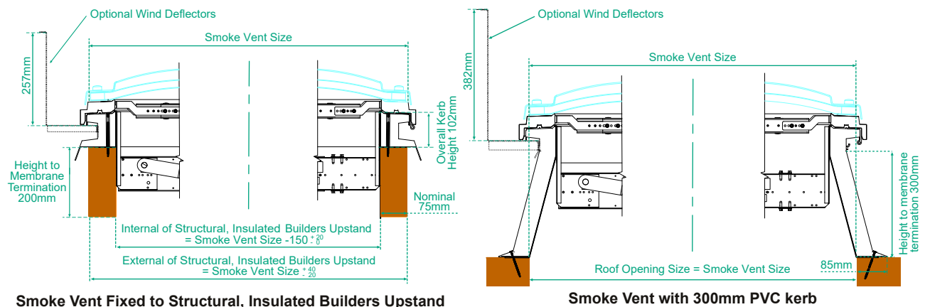
Smoke Vent Fixed to Structural, Insulated Builders Upstand
